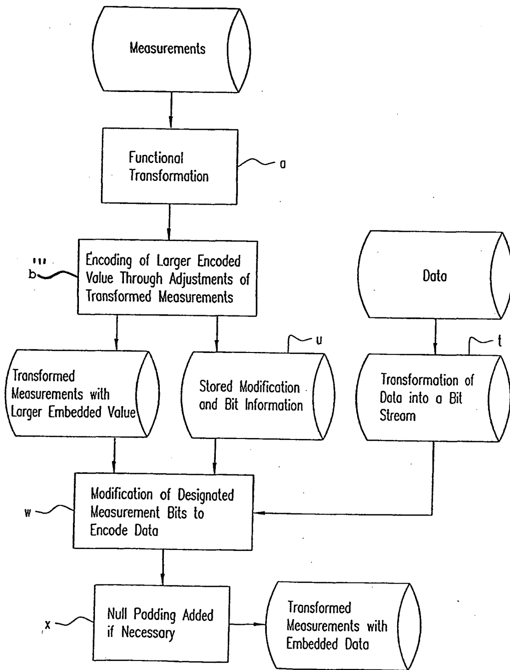
Pre-Computation for Dynamic Embedding
